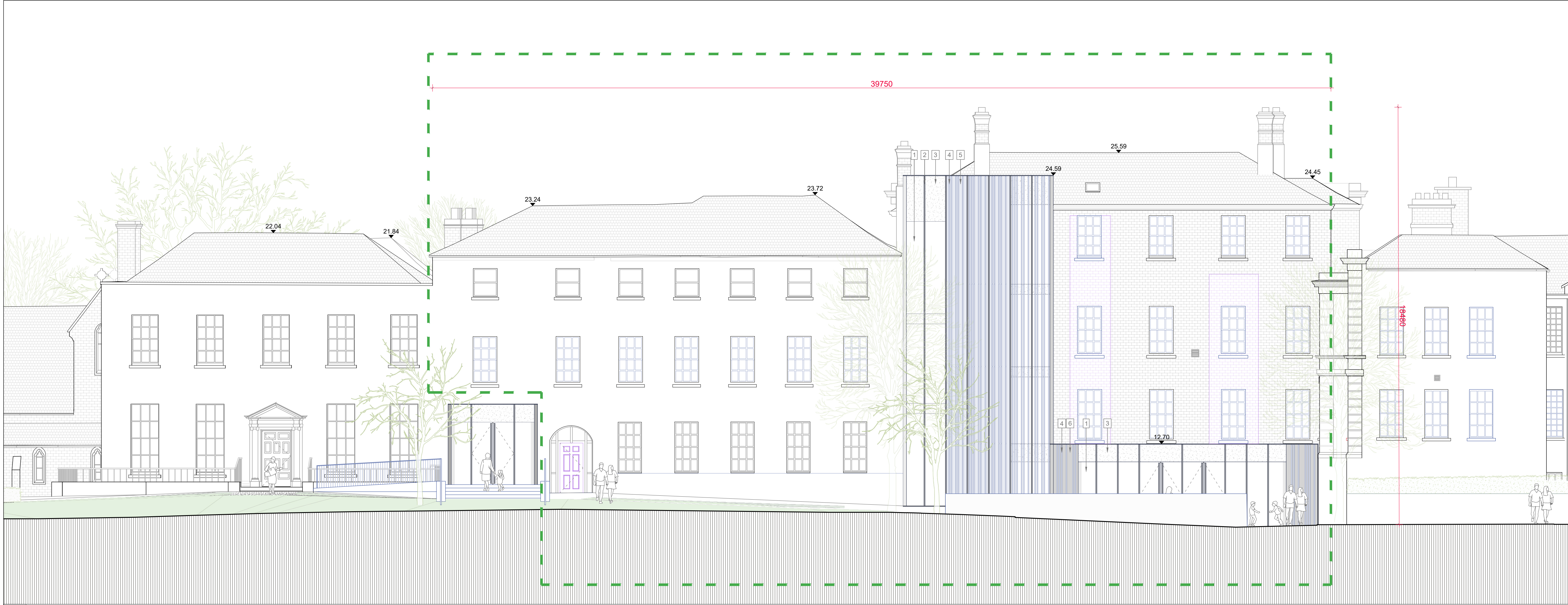
01 North Elevation Proposed SCALE 1:100
