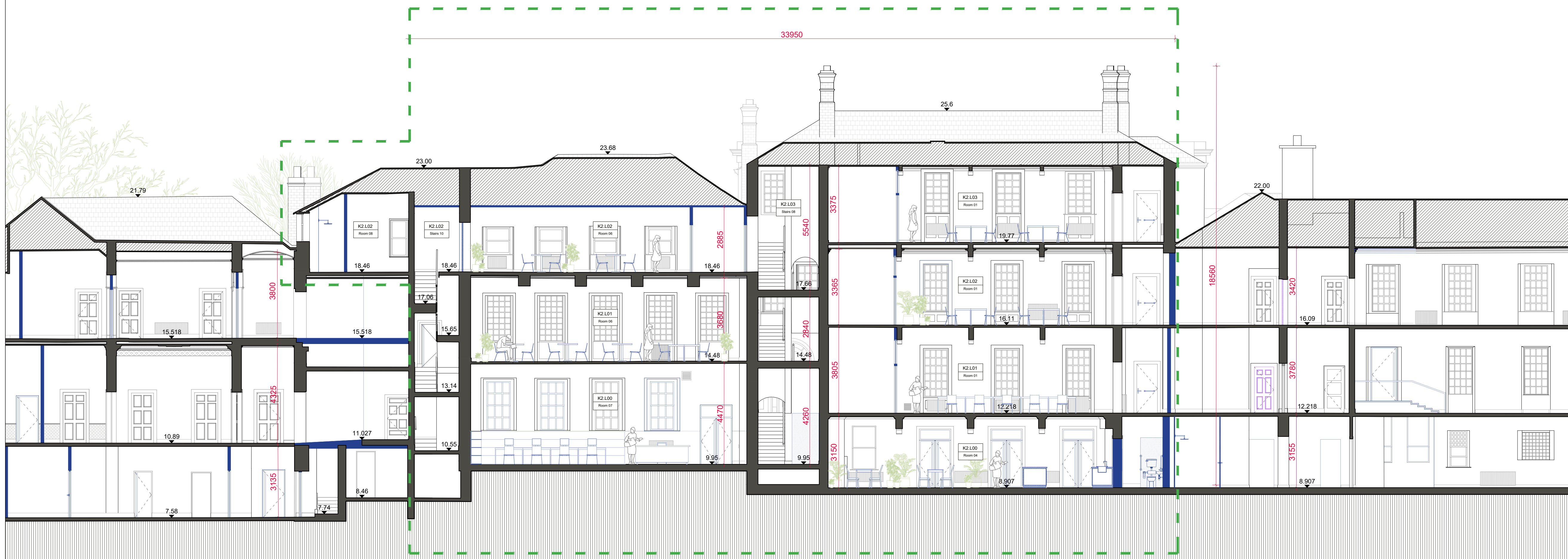
02 Section A Proposed SCALE 1:100
