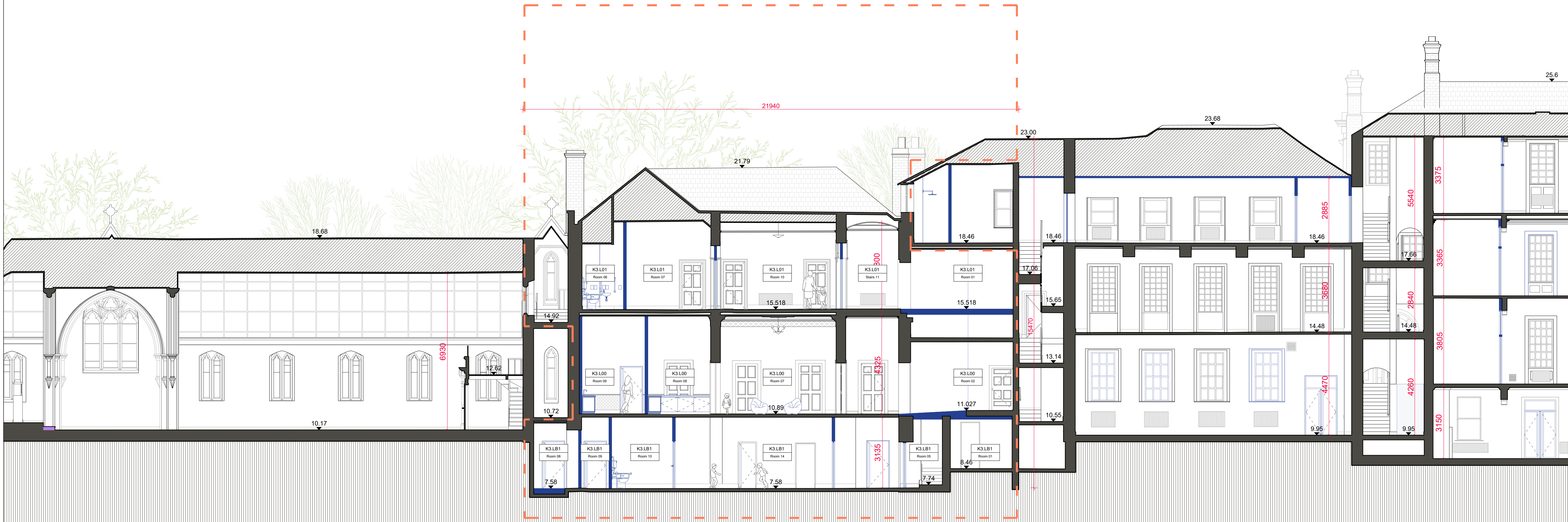
02 Section A SCALE 1:100
