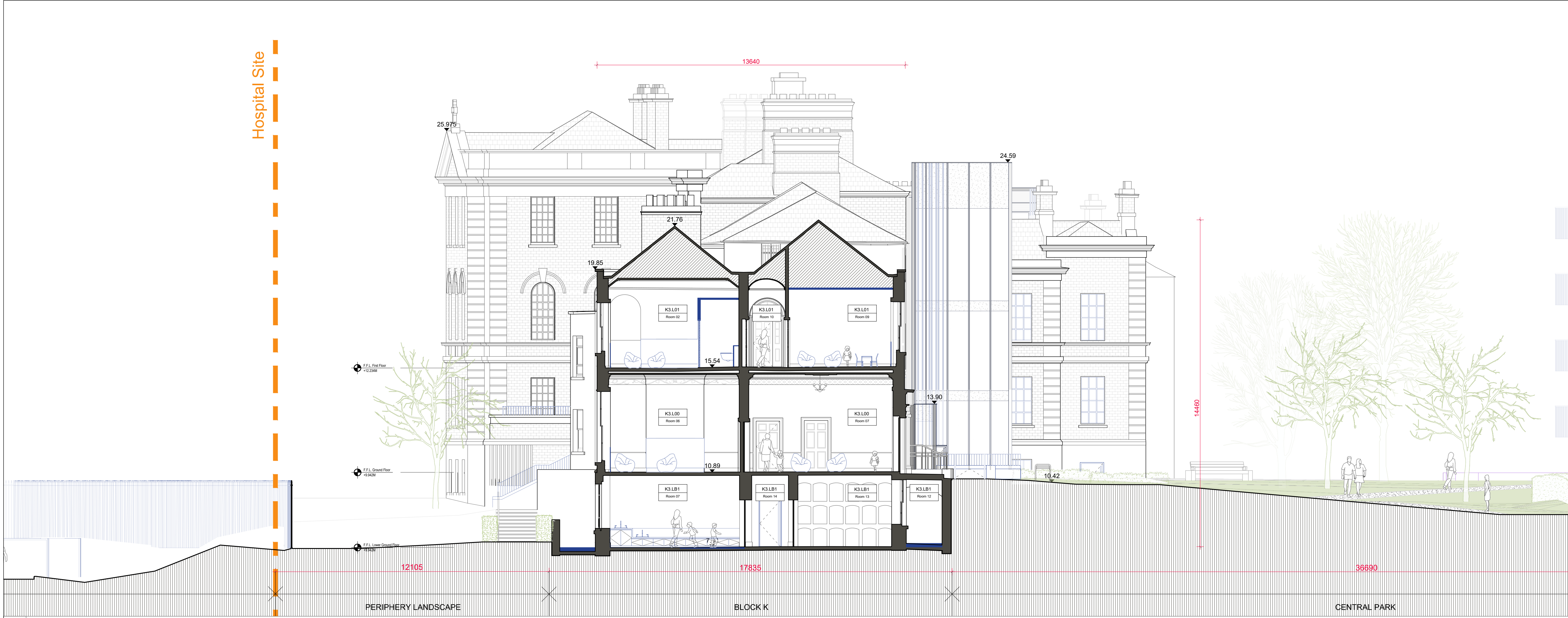
01 Section I SCALE 1:100
