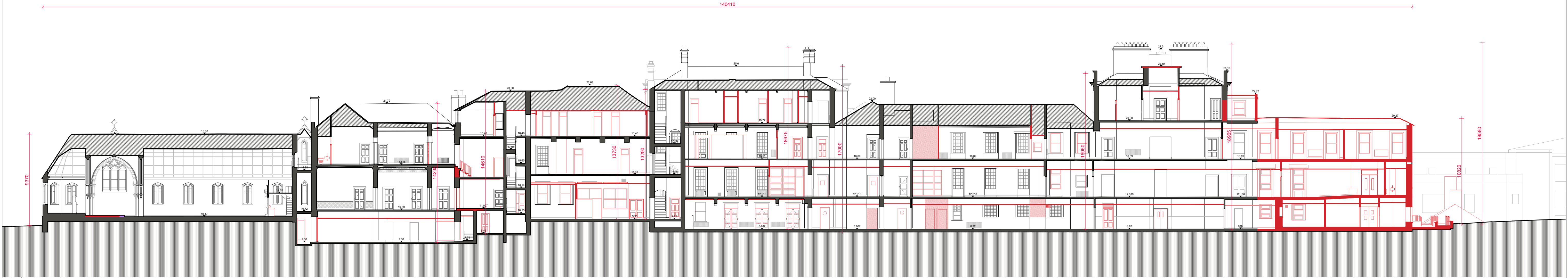
01 Section A Demolition SCALE 1:200
