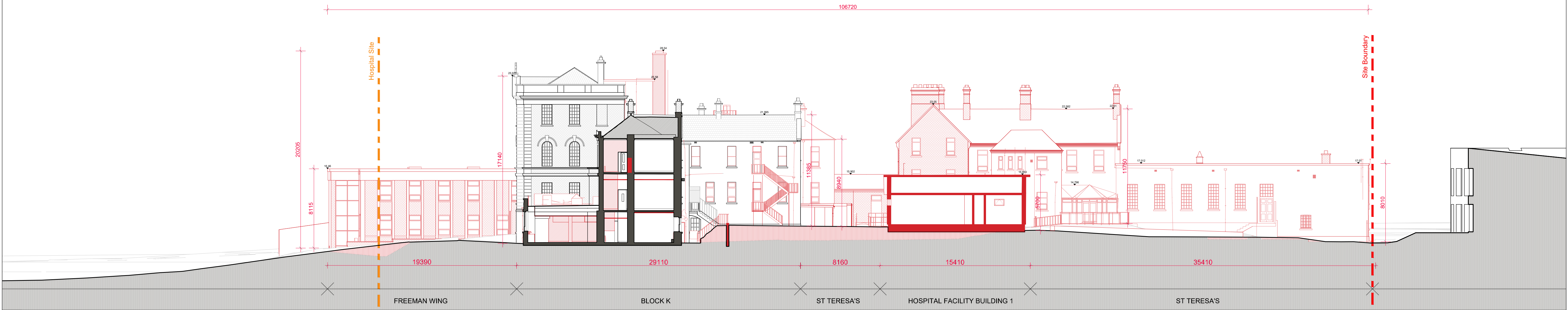
01 Section D - Demolition SCALE 1:200
