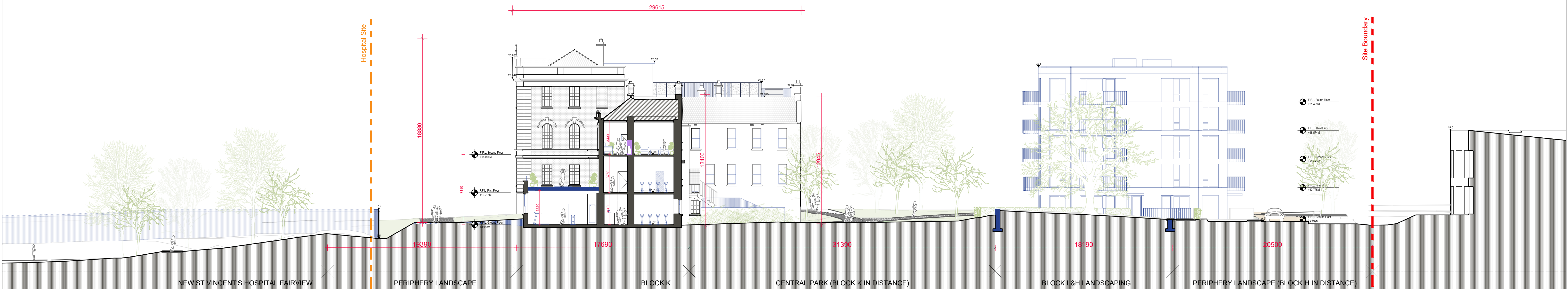
02 Section D - Proposed SCALE 1:200
